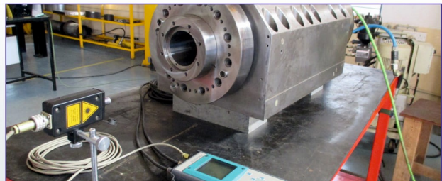
Spindle Balancing
